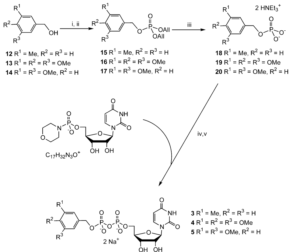
Scheme 3. Reagents and conditions: (i) ( i -Pr 2 N)P(OAll) 2 , 1 H -tetrazol, CH 2 Cl 2 /CH 3 CN (1:1) rt, 2.5 h; (ii) t -BuOOH, 0 °C, 1.5 h, 91% (for 15 ), 82% (for 16 ), 82% (for 17 ); (iii) dimedone, Pd(PPh 3 ) 4 , THF, Et 3 N, rt, 1.5 h, 59% (for 18 ) 70% (for 19 ), 44% (for 20 ); (iv) 1 H -tetrazol, py, rt, 3 days; RP-18; (v) Amberlite IR-120 (Na + -form) 69% (for 3 ), 22% (for 4 ), 30% (for 5 ).
