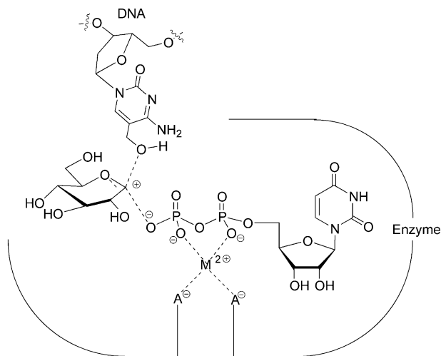
Scheme 1. Postulated transition-state for the sugar transfer catalysed by BGT.
