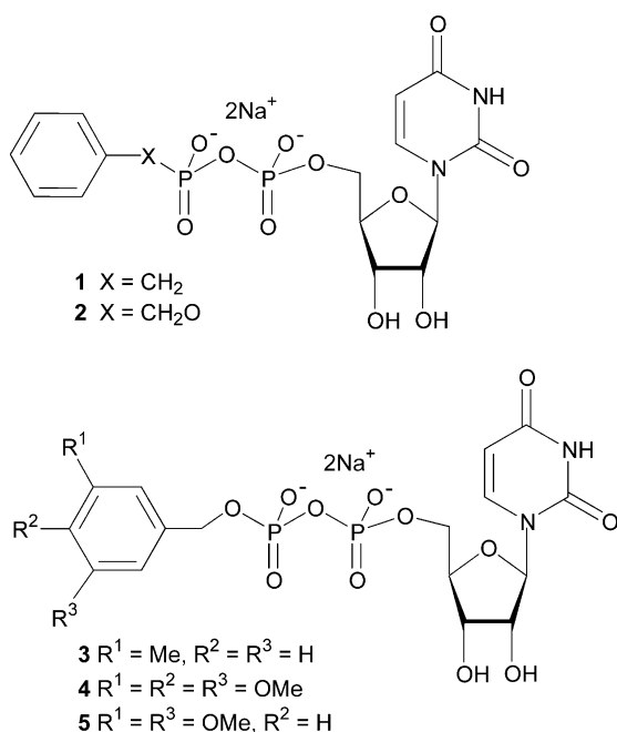
Figure 2. Structures of designed inhibitors 1–5.
