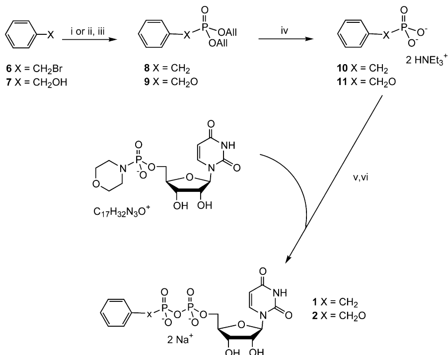
Scheme 2. Reagents and conditions: (i) (AlO) 3 P, toluene, 95 °C, quant (for 8 ); (ii) ( i -Pr 2 N)P(OAll) 2 , 1 H -tetrazol, CH 2 Cl 2 /CH 3 CN (1:1), rt, 2.5 h; (iii) t -BuOOH, 0 °C, 1.5 h, 92% (for 9 ); (iii) dimedone, Pd(PPh 3 ) 4 , THF, Et 3 N, rt, 1.5 h, 50% (for 10 ), 60% (for 11 ); (iv) 1 H -tetrazol, py, rt, 3 days; RP-18; (v) Amberlite IR-120 (Na + -form), 88% (for 1 ), 77% (for 2 ).
