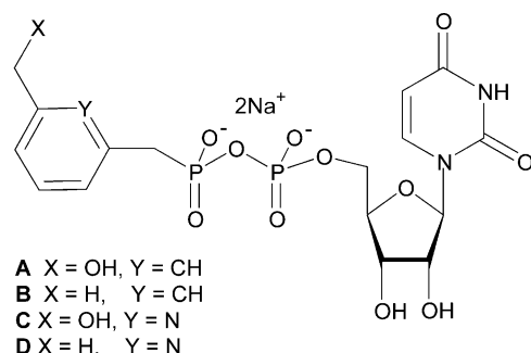
Figure 1. Reported inhibitors A–D.
